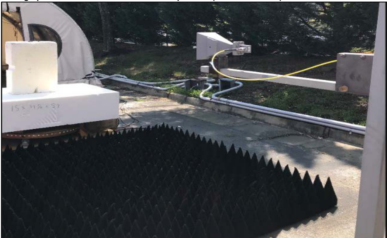
Photograph 6: Radiated Emissions Test Setup – Rear (Above 1000 MHz)
