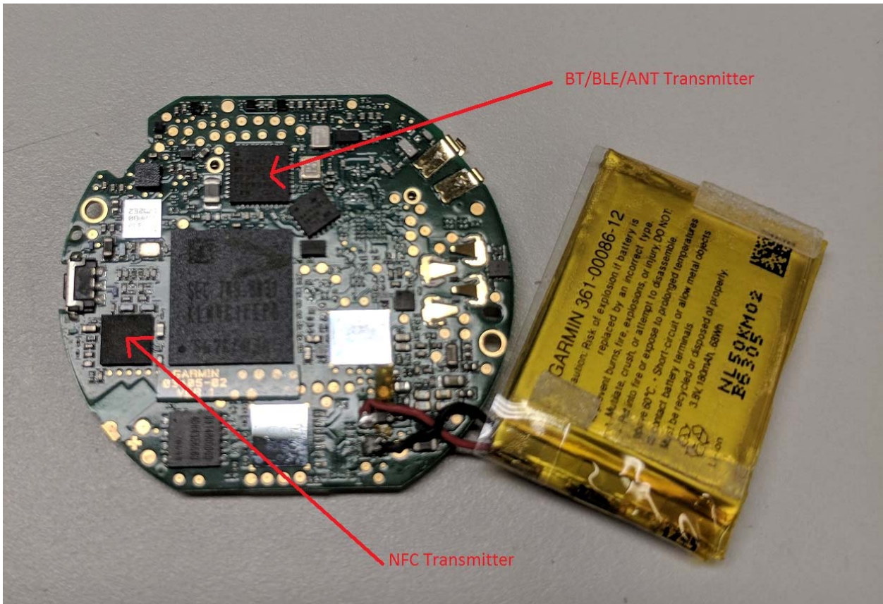
Bottom side of PCB [battery removed]
