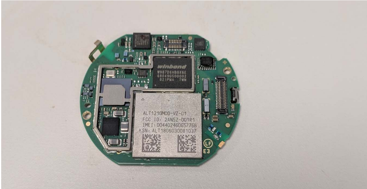
Top side of PCB [shield cover removed]
